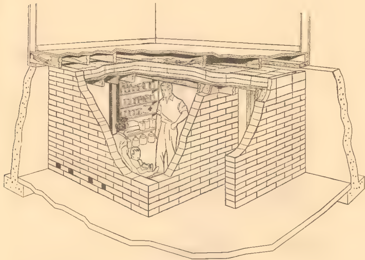
Figure 7.—Basement Concrete Block Shelter
