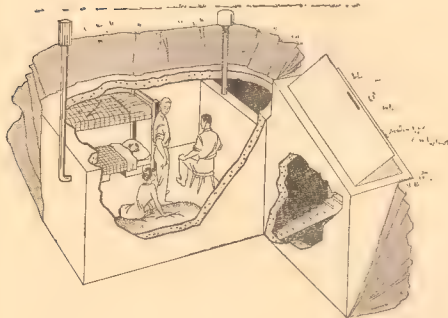
Figure 12.—Concrete basement shelter in new housing
