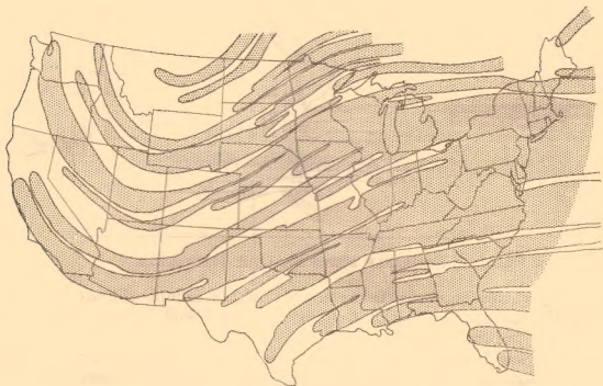
Figure 2.—Fallout areas at 24 hours after detonation
