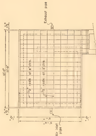
ROOF PLAN SHOWING REINFORCING
