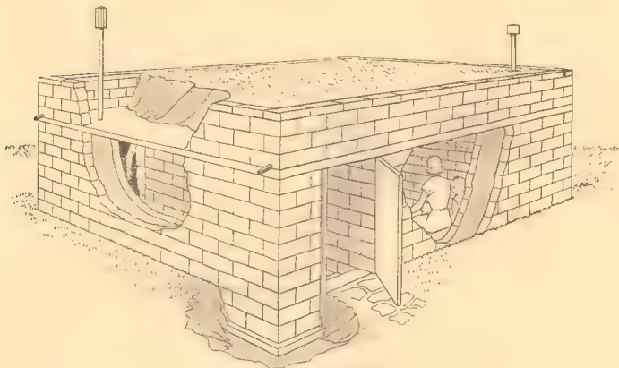
Figure 9.—Aboveground double-wall shelter
